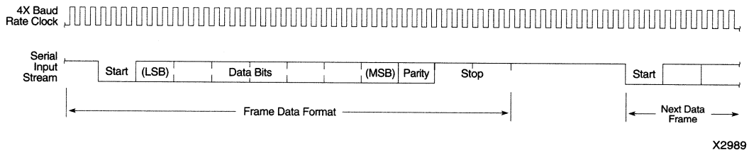
Figure C-2 UART Waveforms
