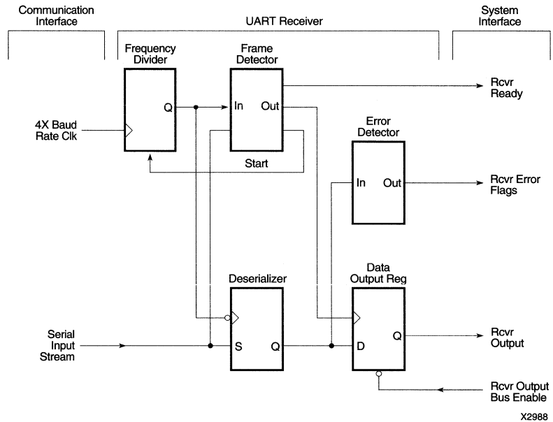
Figure C-1 UART Receiver Functional Logic Diagram
