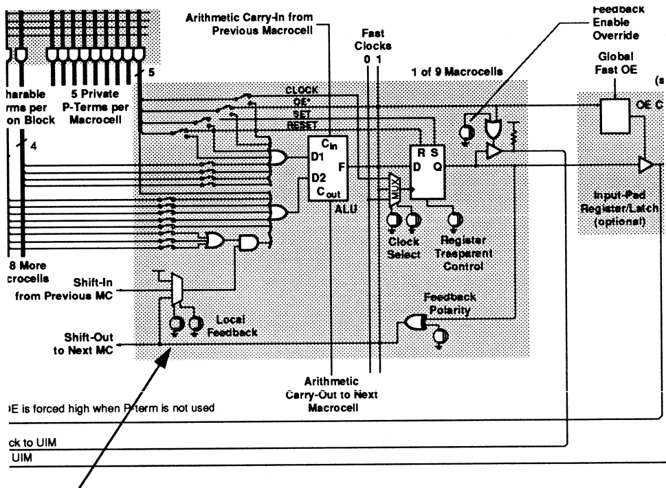
High Density Function Block Schematic
